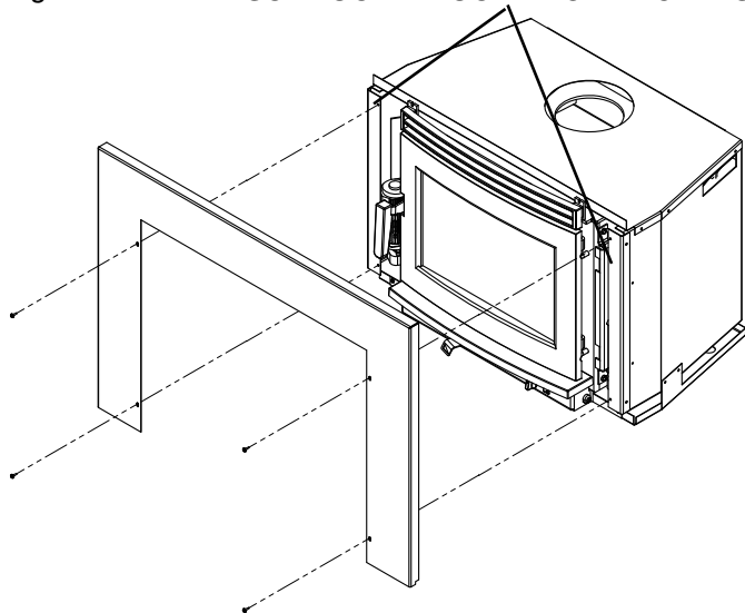
Fig. # 7 SURROUND MOUNTING BRACKETS
