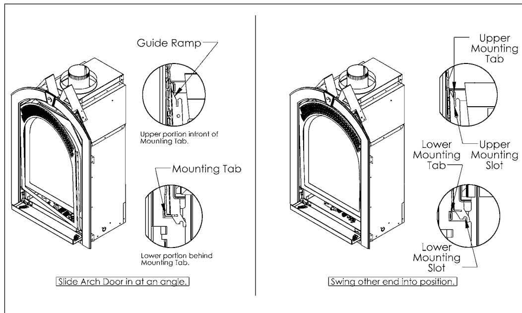
Figure 16 - Arch Door mounting tab locations.
