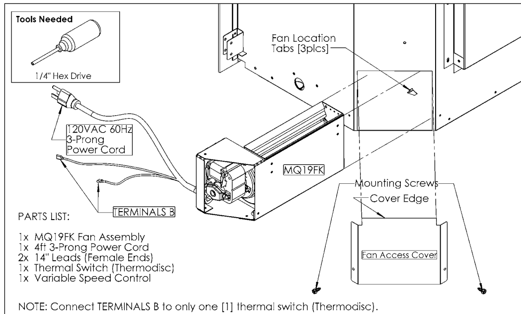
Figure 18 - Optional Fan Kit installation.
