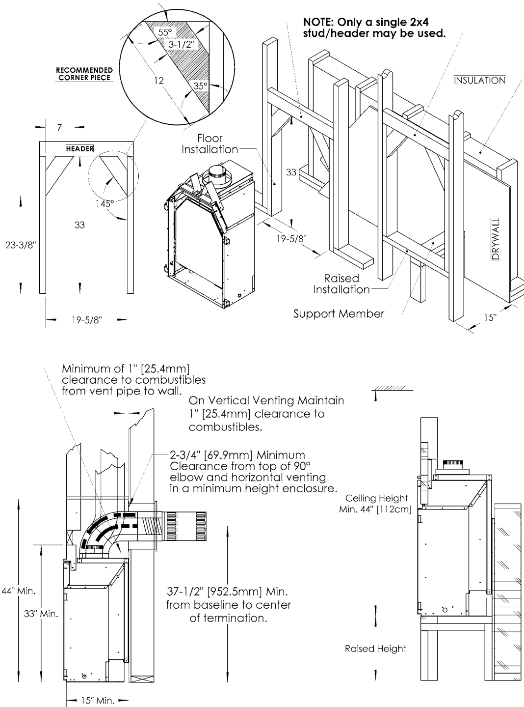
Figure 5 - General framing installation.
