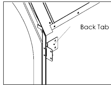
Figure 4 - Cabinet mount configuration.
