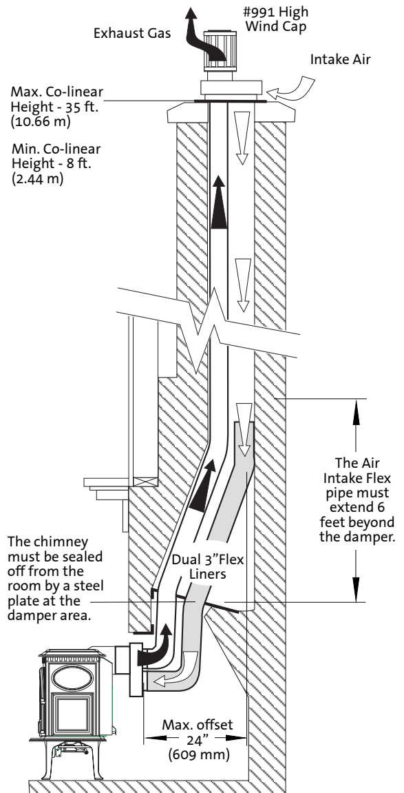
Figure 14. Co-linear Adaptor installed through a masonry chimney. Simpson Dura-Vent components shown.
