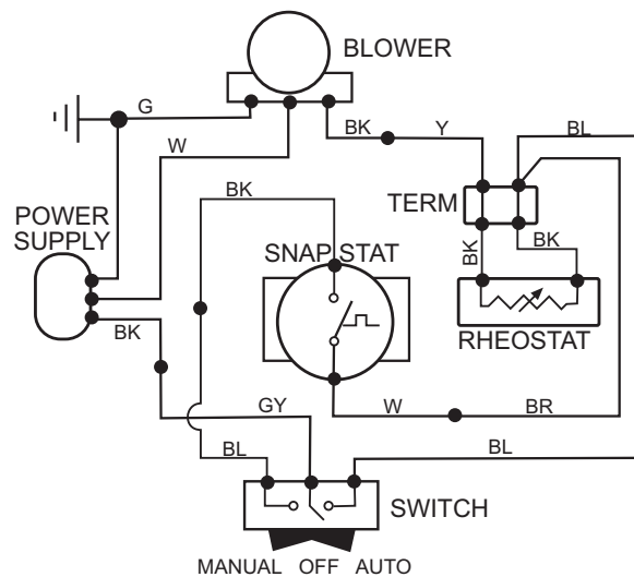
Figure 46 . Blower Wiring Diagram
