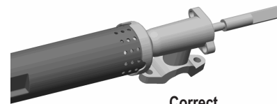
Correct burner-to-valve engagement
